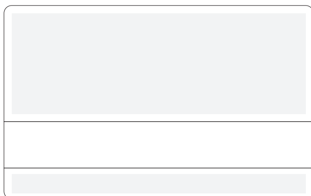
LabelTag 80 x 50mm Printable area 76 x 26mm Bottom printable area 76 x 5mm
